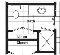
AVAILABLE ALTERNATE BATH LAYOUT FOR MAIN FLOOR POWDER ROOM
