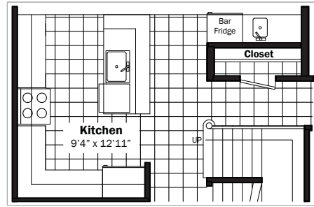
AVAILABLE ALTERNATE KITCHEN
